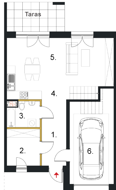
PARTER
